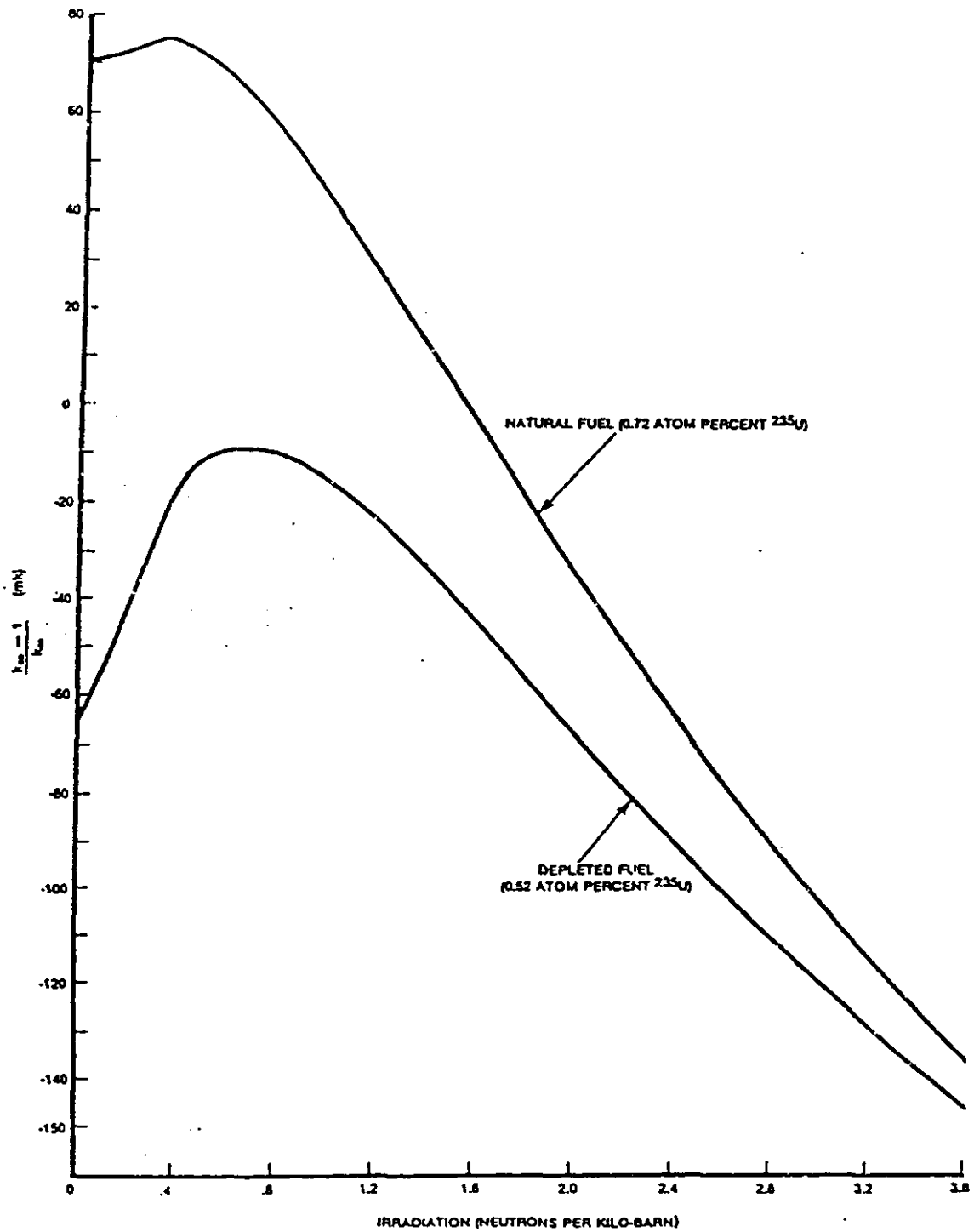
Figure 4.2 Reactivity versus Irradiation of Natural and Depleted 37-Element Fuel
