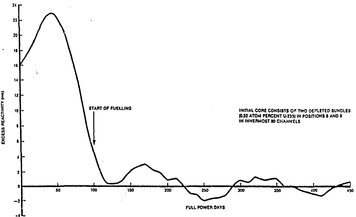
Figure 4.4 Variation of Excess Reactivity During Initial Burnup Period (FIMDP Simulations)
