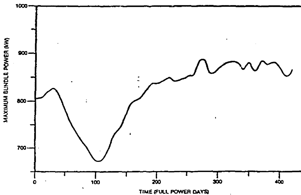
Figure 4.10 Maximum Bundle Power
