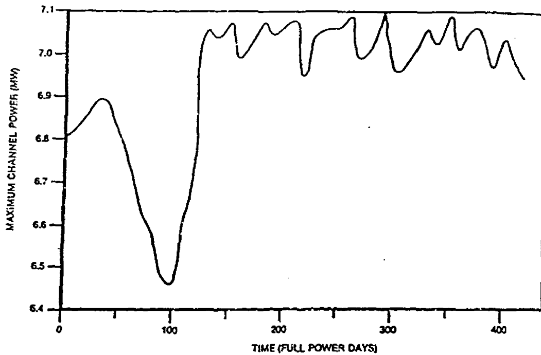
Figure 4.9 Maximum Channel Power
